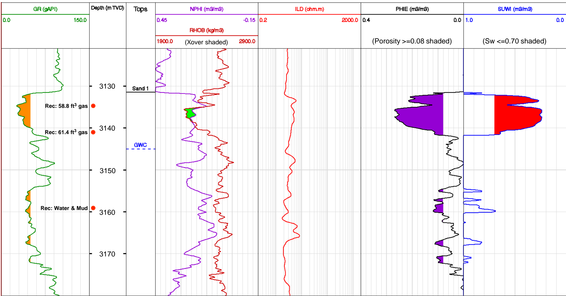
Marmora C-34 - Sand 1 (Top Missisauga) Petrophysical Results Plot. The position of wireline tester samples (red dots) and the gas-water contact (GWC) are shown.
